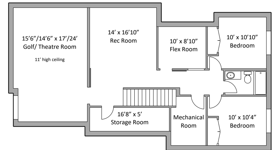
1210 sq ft future basement development
