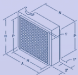
F200A FILTER SECTION For IDB, IDB-X, 200 & 9200 Series Duct Blowers
