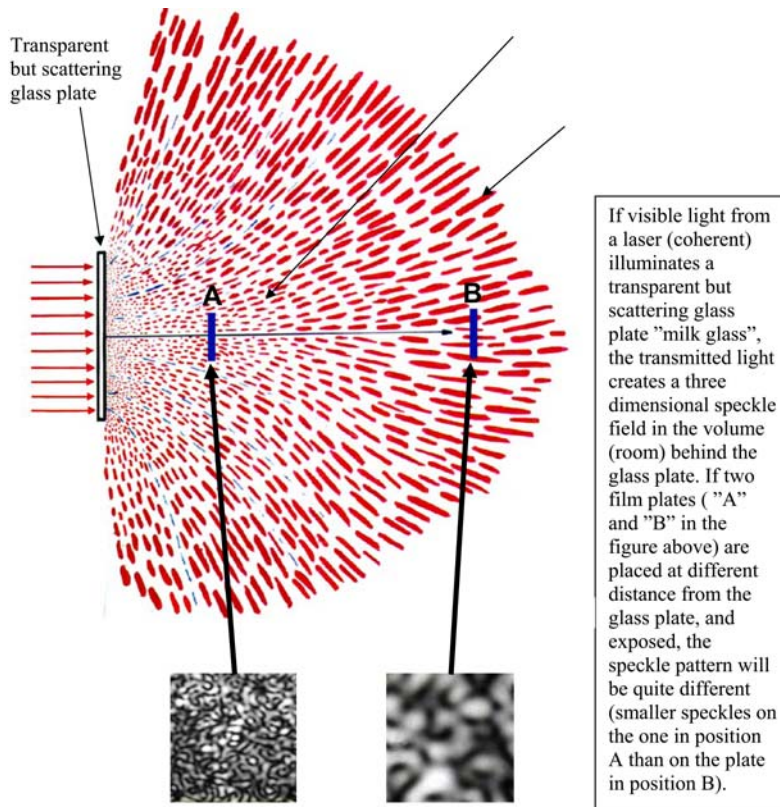
Figure 1.16 Speckle pattern
