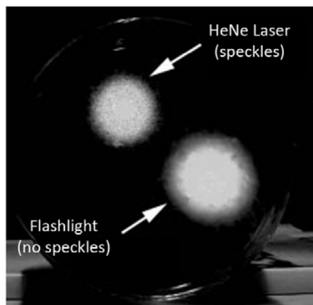
Figure 9.2 Light spots on the back side of a slab of minced meat through which the light from a HeNe laser and a flashlight has penetrated. The upper left spot originates from the HeNe laser, and the lower right spot originates from the flashlight. Both spots are red after their passage through the meat, which shows that red light has the best penetration of the visible light wavelengths. Infrared radiation penetrates even better. The figure shows that coherence of the laser light is not lost as the light penetrates the meat. The laser speckles can be clearly seen, and it is obvious that there is a difference between laser light and the light from a flashlight.
