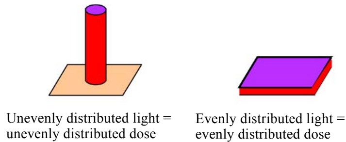
Figure 10.13 Distributed light
