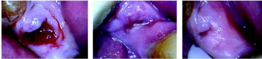
Figure 5.6 Same patient, contra-lateral side; with red laser treatment directly postop, at 15 and 30 days. Courtesy: Talat Qadri
