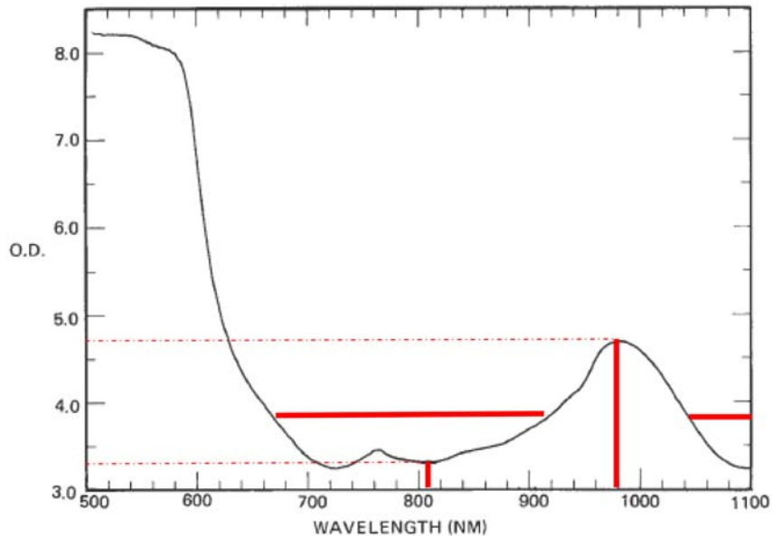
Figure 2.3 The absorption spectrum of a human hand. This spectrum was recorded with a very sensitive spectrophotometer with the hand in close juxtaposition with the photocathode (unpublished data of Karl H. Norris, from The Science of Photobiology , KC Smith, ed., Plenum Press, 1977; p. 400).
