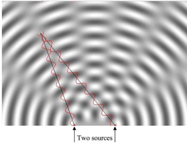
Figure 1.13 Interference pattern
