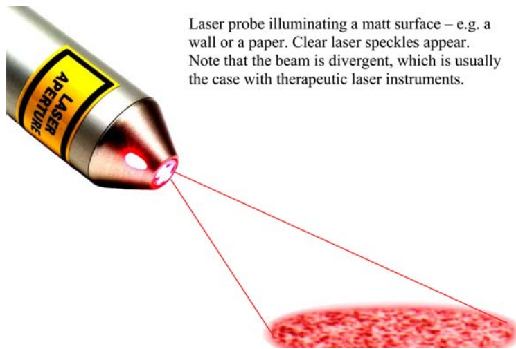
Figure 1.14 Laser speckles
