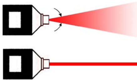
Figure 1.20 Collimation
