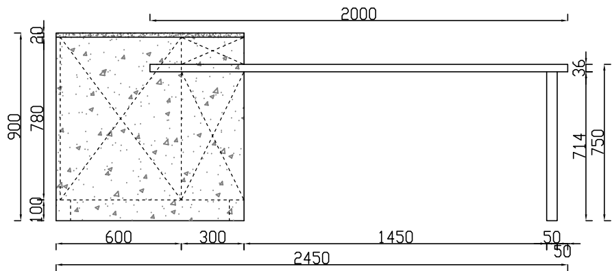
ELEVATION C
