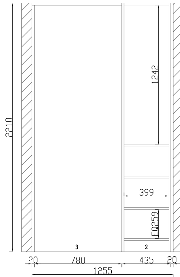
ELEVATION C
