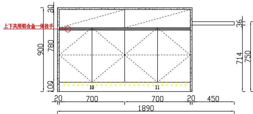
ELEVATION D
