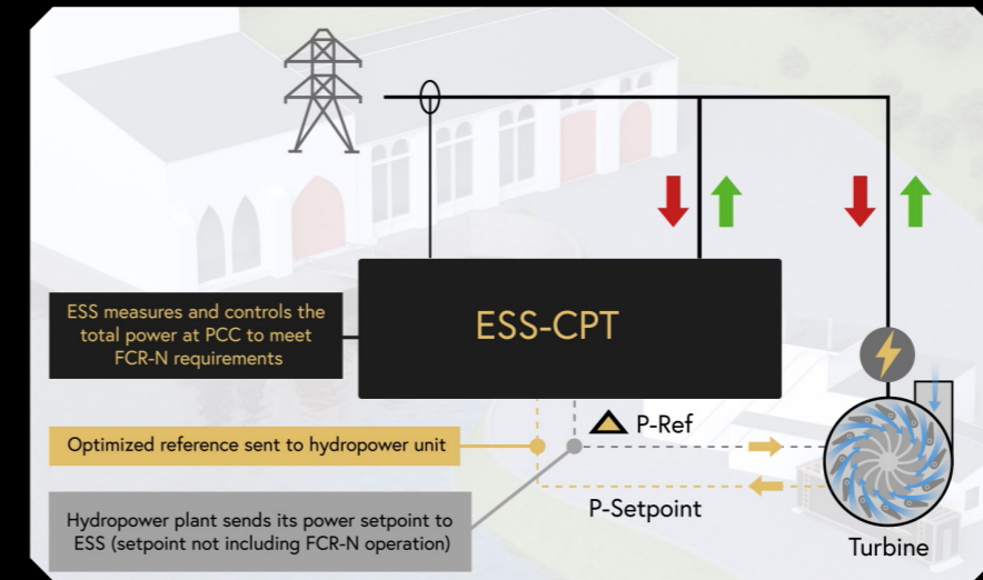
Combined Hydropower + Energy Storage System
