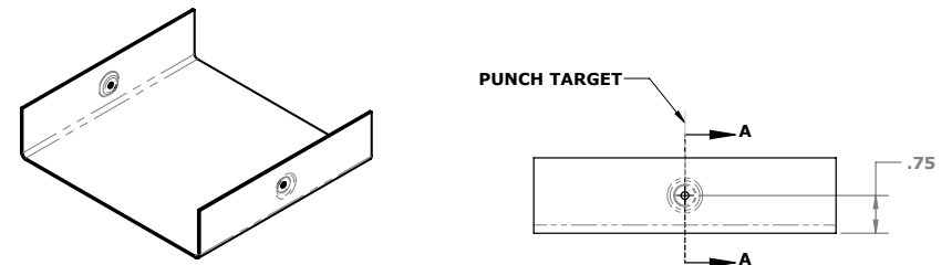
Flange Dimple
