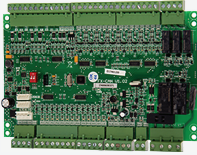
ARKEL FX-CAN [ARKEL FX-CAN]
