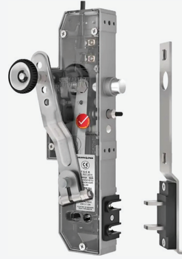
YARI OTOMATİK KAPI KİLİDİ [SEMI-AUTOMATIC DOOR LOCK]
