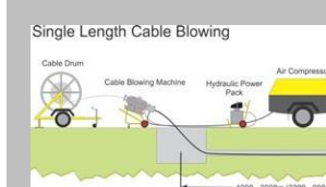
CABLE BLOWING
