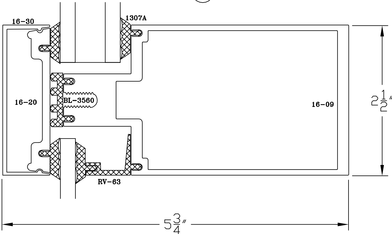
②A HORIZONTAL
