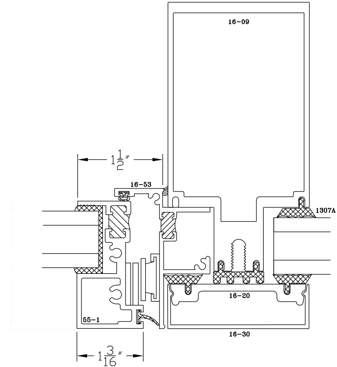
LOW PROFILE VENT
