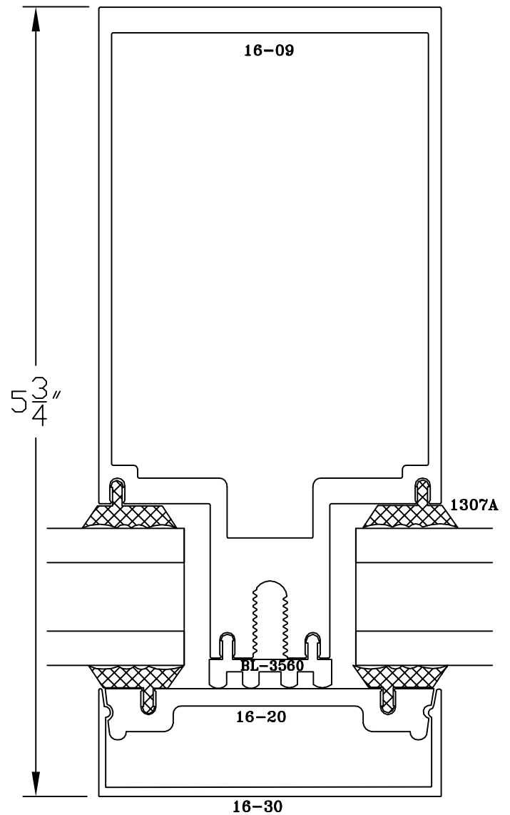
⑧A VERTICAL
