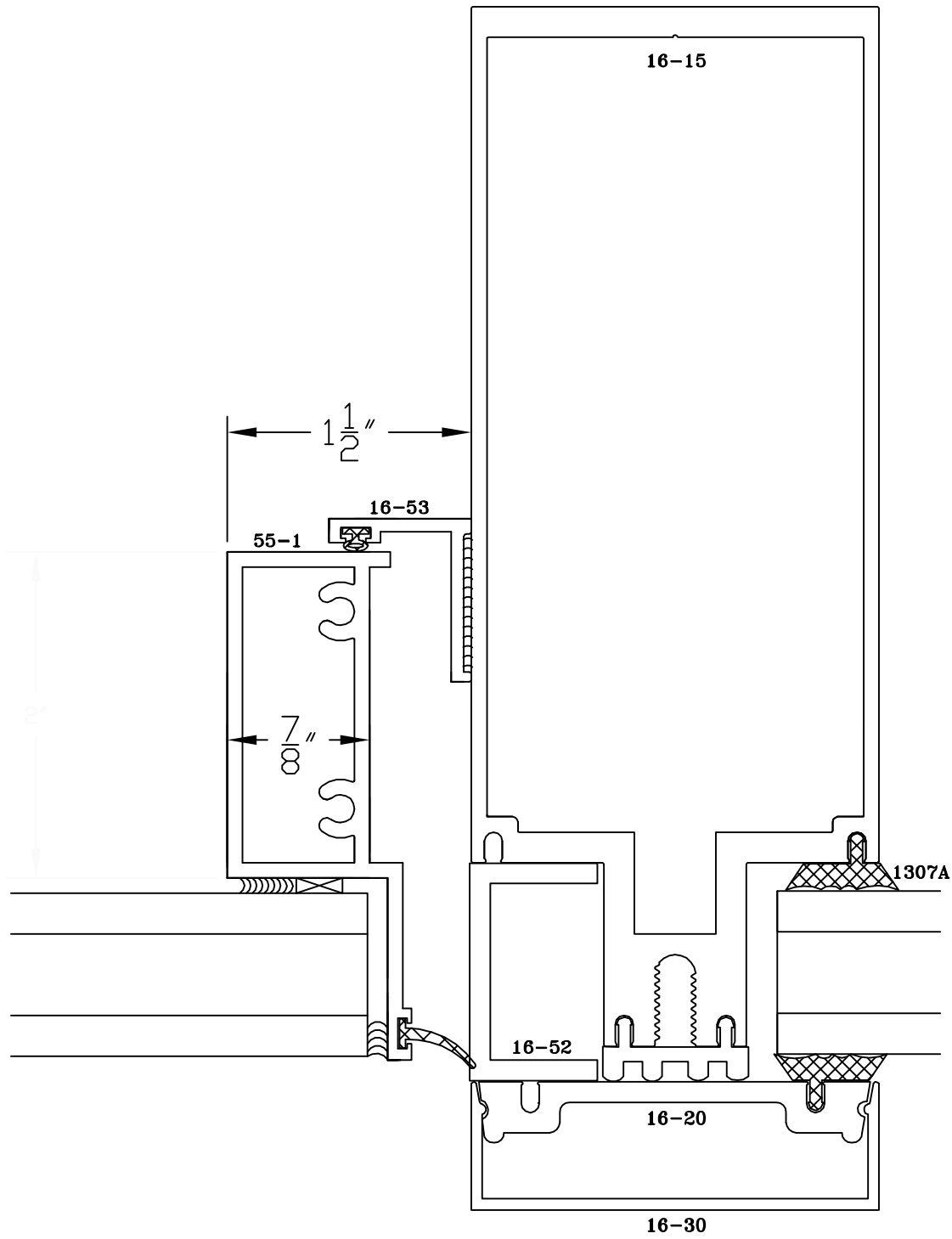
CONCEALED CURTAINWALL VENT
