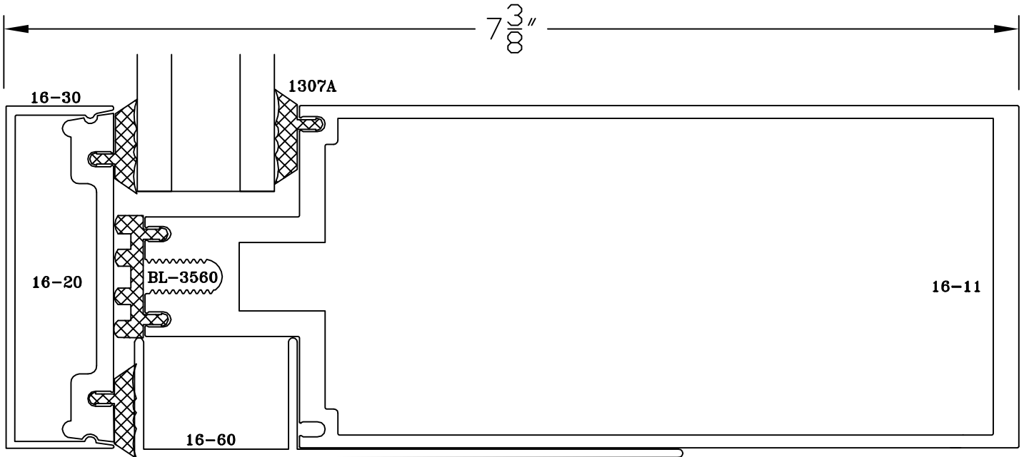
⑥ SILL
