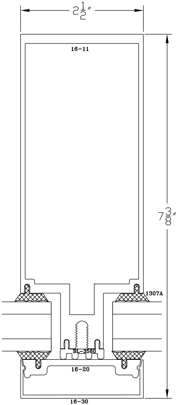
⑧ VERTICAL
