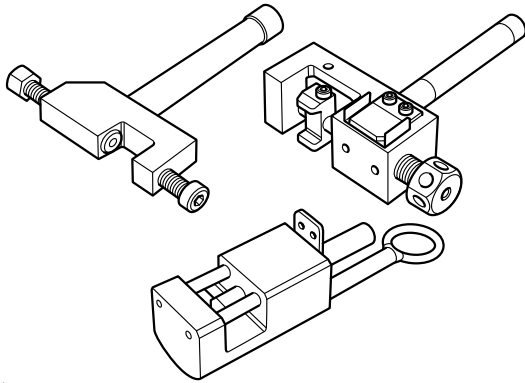
T3880205 - Kit Chain Link Tool (Regina Chain)
