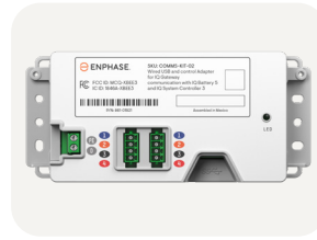
COMMS-KIT-02 Enphase Communications Kit Enables wired communications using Control cables for systems not using IQ Combiner 5/5C.
