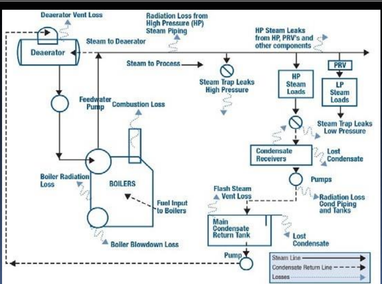
Boiler & Steam System Losses. Source: energy.gov
