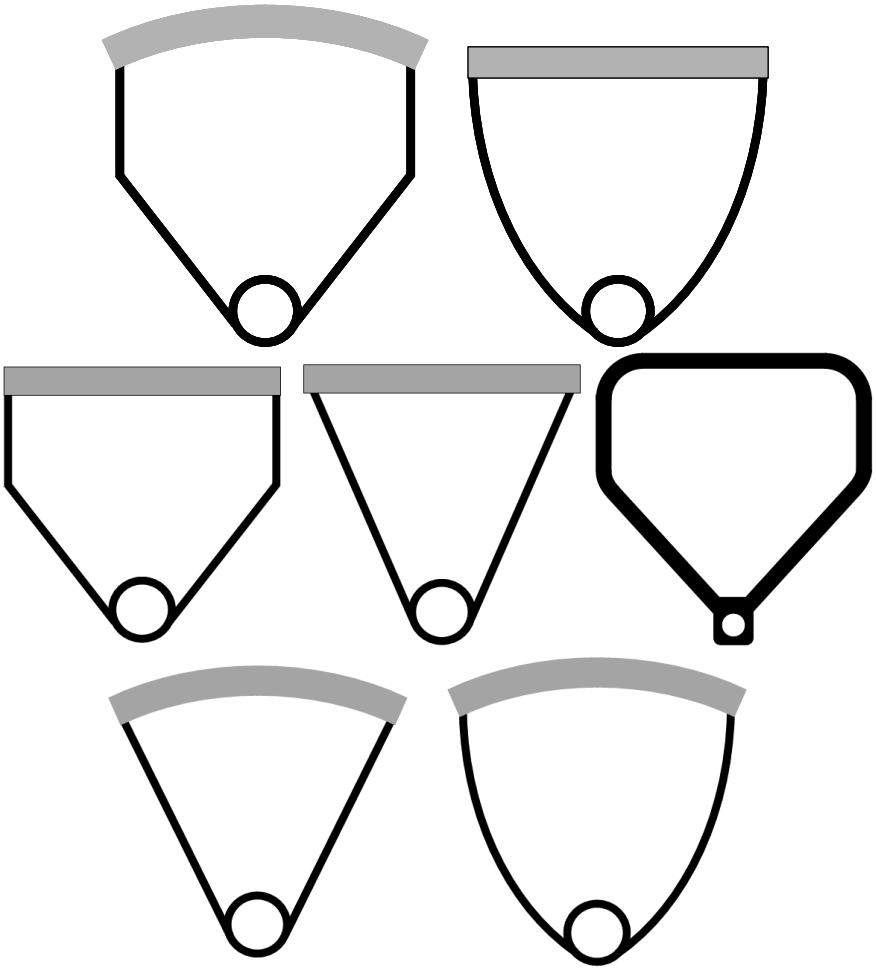
FIGURE 14 – HAMMER HANDLE
