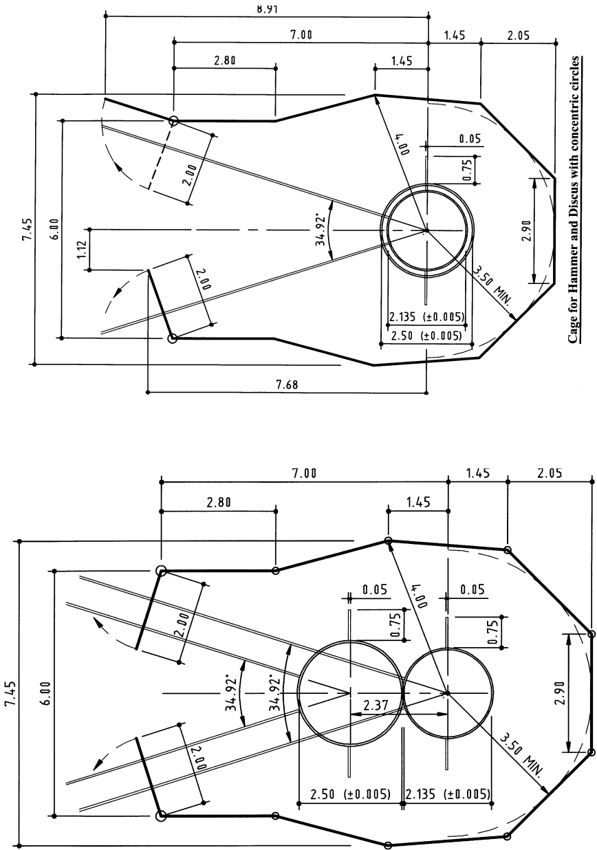
FIGURE 12 – IAAF HAMMER/DISCUS CAGE LAYOUTS
