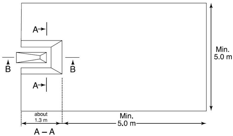
Plan of a Suitable Landing Area
