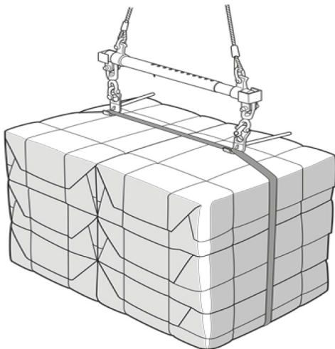
Figure 65. Lifting banded unitized loads
