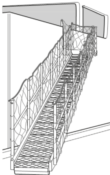
Figure 96. Accommodation ladder with a safety net
