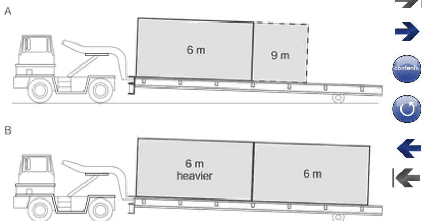
Figure 87. Distribution of load on a roll trailer
