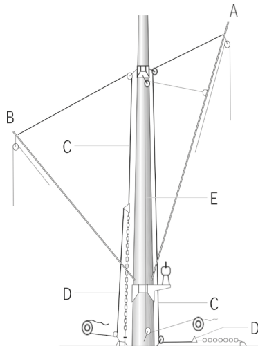
Figure 32. Ships' lifting appliances – A ship's derrick with topping lift and pendant
