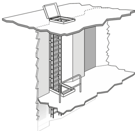
Figure 101. Hold ladder
