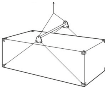
Figura 78. Bottom lifting of containers
