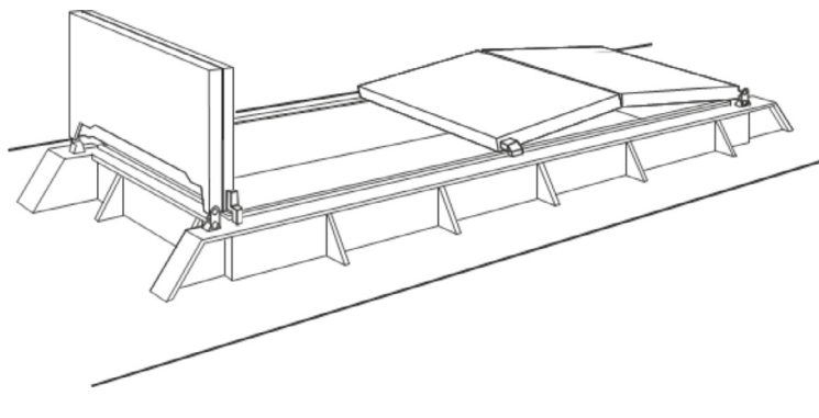
Figure 102. General arrangement for a rolling/sliding hatch cover
