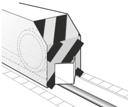
Figure 35. Rail-mounted crane wheel protection
