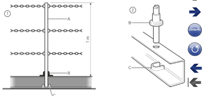
Figure 104. Moveable fencing for 'tween decks (locking device omitted for clarity)
