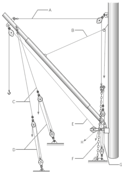
Figure 33. Rigging of ship's derrick boom
