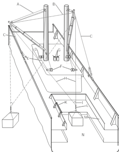
Figure 54. Derricks in union purchase rig
