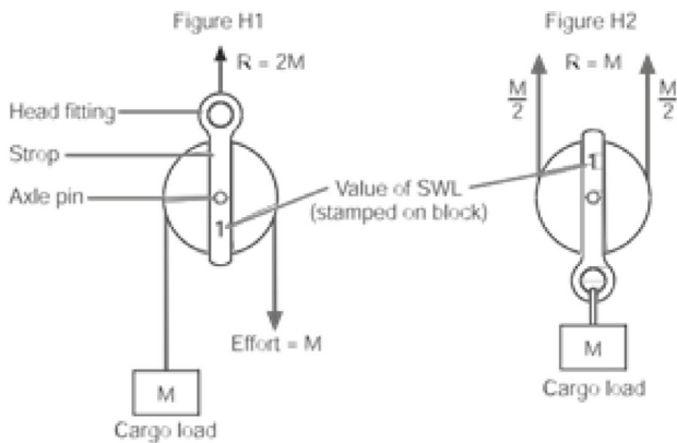
Figure 47. Safe working loads of single-sheave blocks
