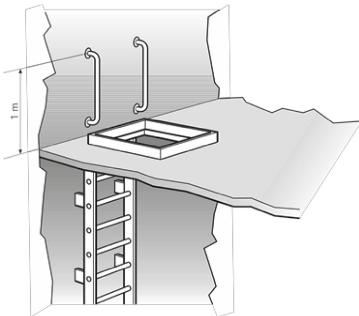
Figure 15. Vertical ladder through opening (figures may not show all appropriate safety equipment and are for illustrative purposes only)
