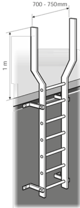
Figure 16. Vertical ladder rising above edge
