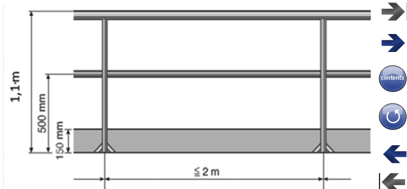
Figure 8. Construction of fencing
