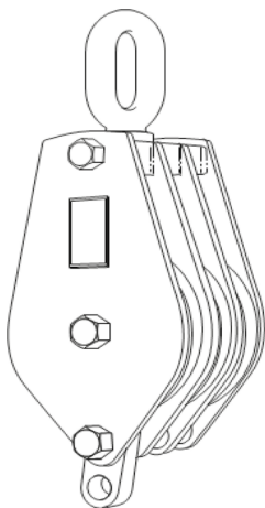
Figure 46. Three-sheave block with becket
