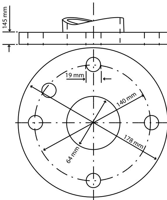
Figure 2. Shore connection for international ship–shore fire connection
