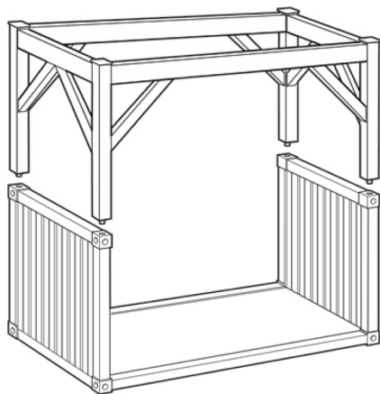
Figure 79. Over-height frame
