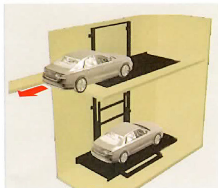
7. Removing car on Top Platform before lifting lower car Option: if garage has some sufficient space car can also be lifted
