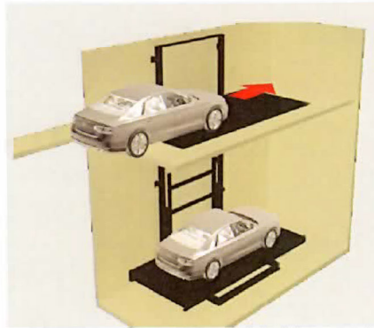
5. Both Platforms receive vehicles
