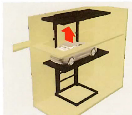
8. Lifting car for removal
