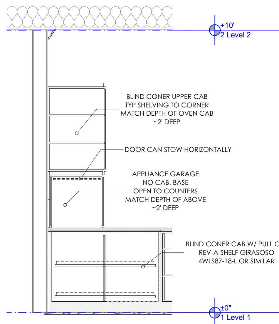
9 MILLWORK SECTION 1 SCALE: 1/2" = 1'-0"
