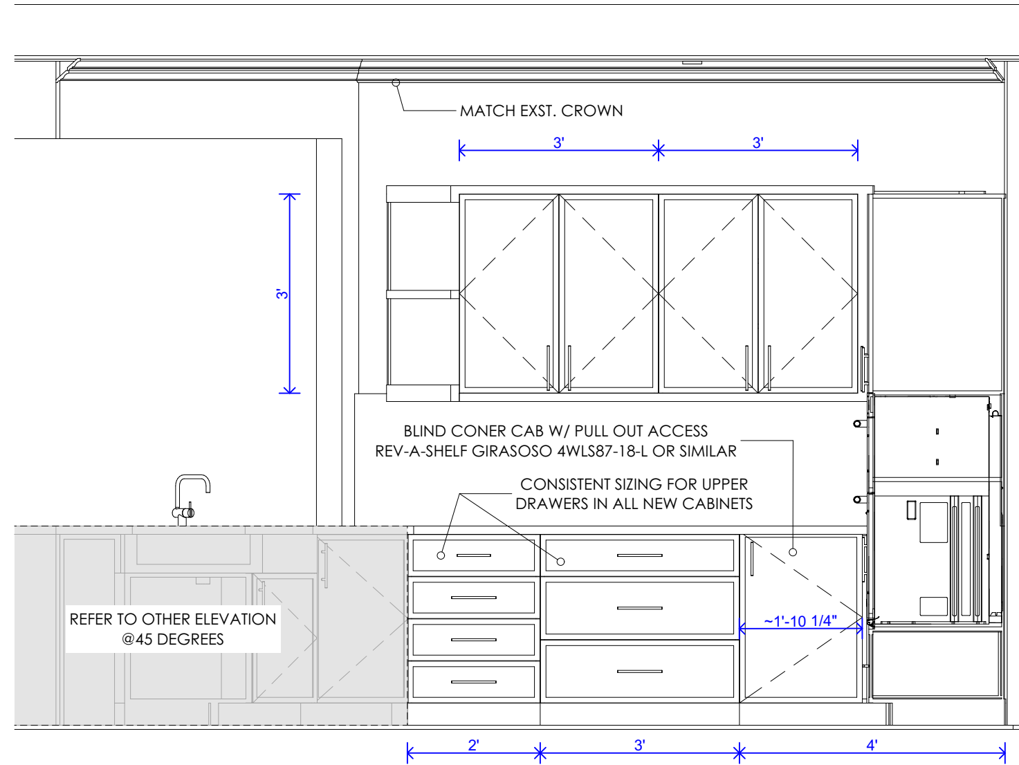
2 IE KITCHEN UPPERS WALL SCALE: 1/2" = 1'-0"
