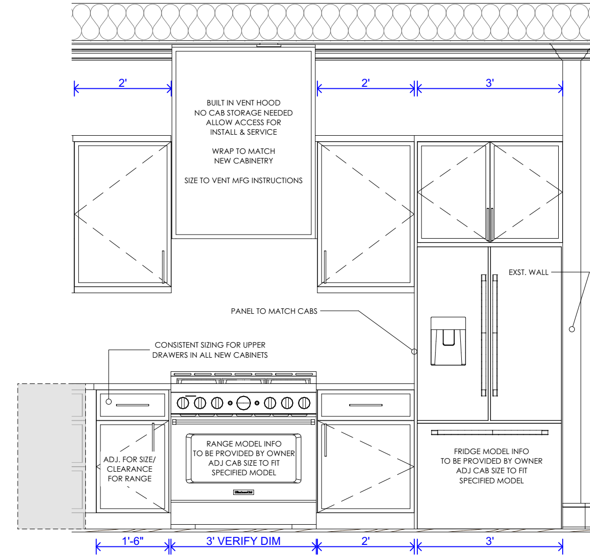
4 IE KITCHEN FRIDGE/ STOVE SCALE: 1/2" = 1'-0"
