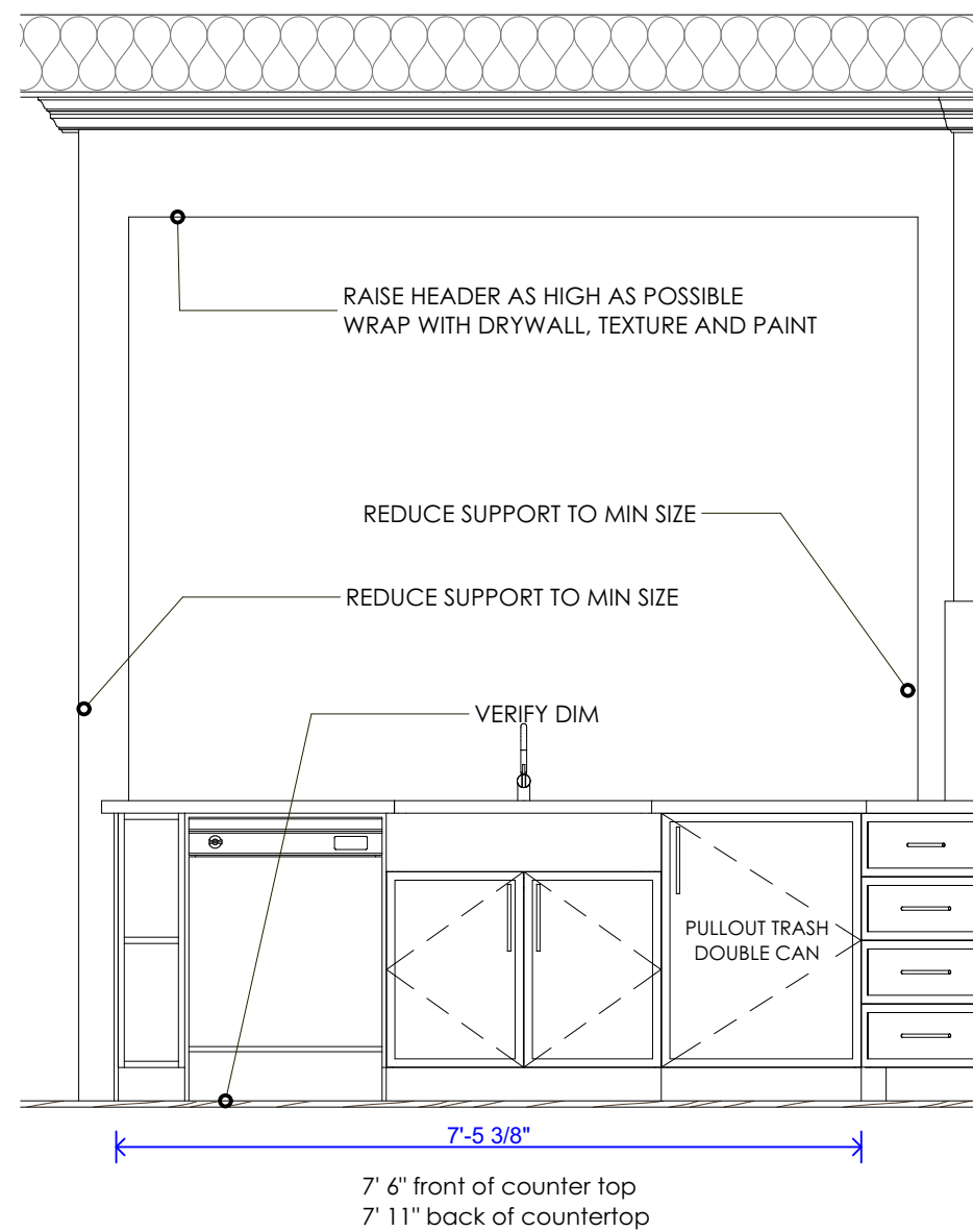
1 IE KITCHEN COUNTER SCALE: 1/2" = 1'-0"
