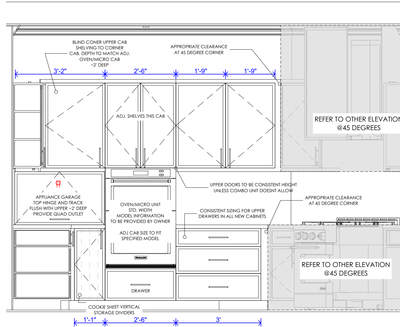
3 IE KITCHEN OVEN SCALE: 1/2" = 1'-0"
