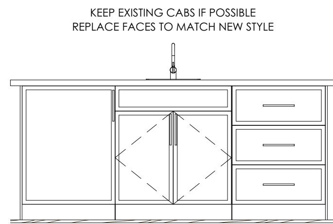
5 IE KITCHEN ISLAND SCALE: 1/2" = 1'-0"
