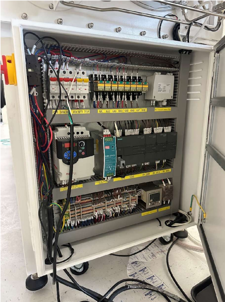
Electrical control cabinet
