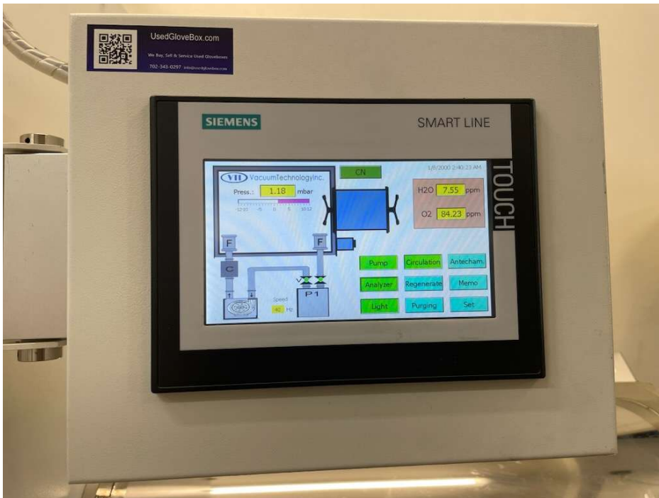
Main control screen showing blower running on compressed air (for testing purposes)
