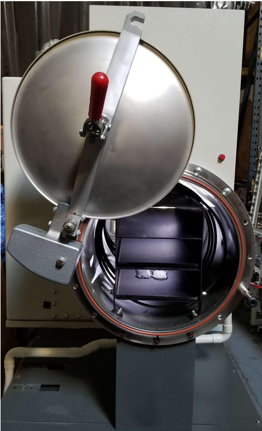
200C Vacuum oven interior showing heating coils and 3 shelf muffle
