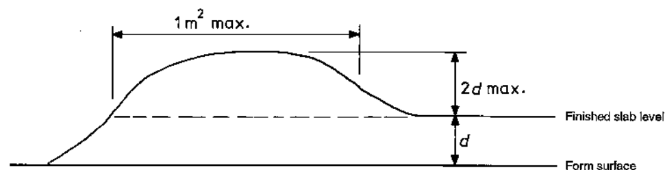
Figure 2. Controlled heaping of concrete
