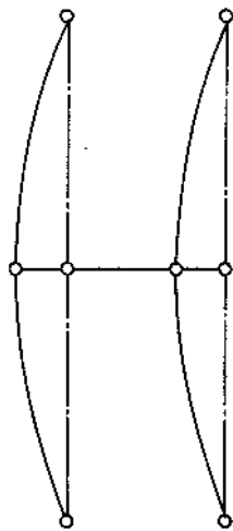
a) Ineffective rotational and positional restraint
