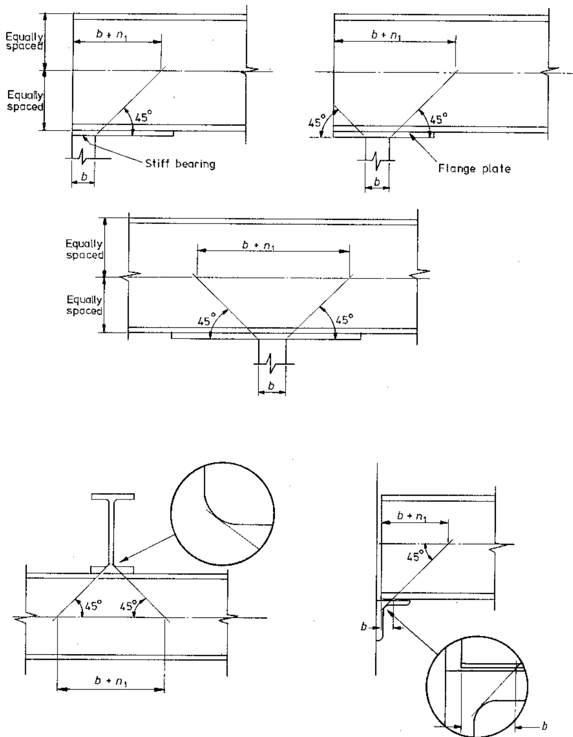
Figure K.1 Stress dispersion: buckling
