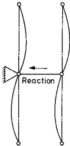
b) Effective positional restraint NOTE. Original position of members shown dashed.
