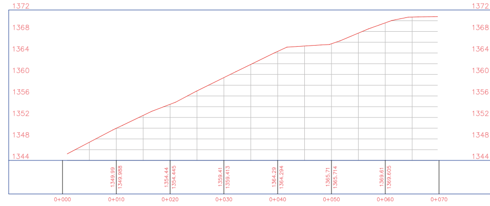
Alignment - (1) PROFILE
