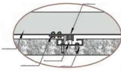
Buried ground rail and the structural profile of the anti-fall device
