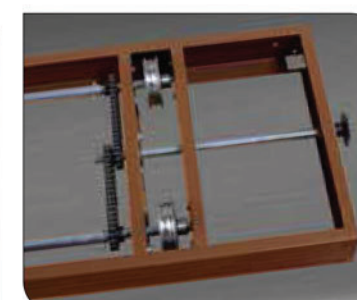
Bottom transmission mechanism
