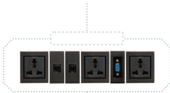
Multifunctional Panel-Bottom case GD-X218-C
