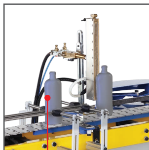
Conical objects
