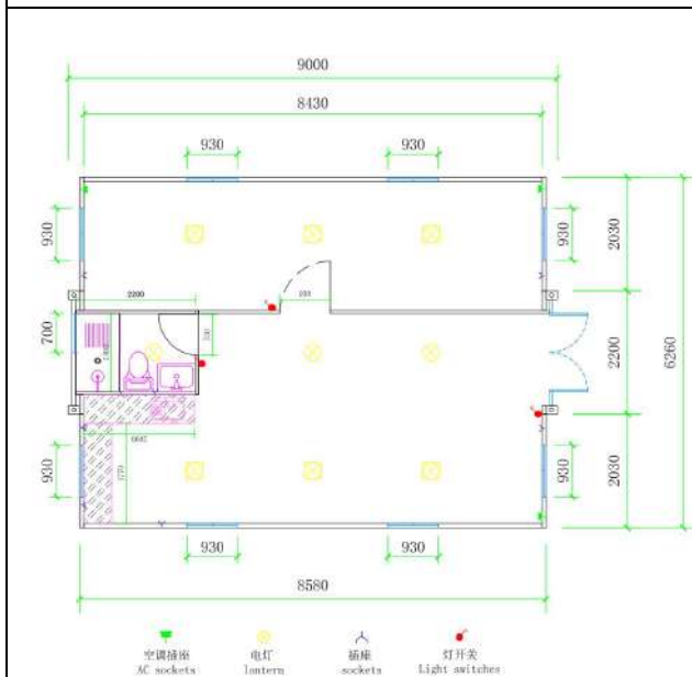
30-foot double-wing expansion room - single room
