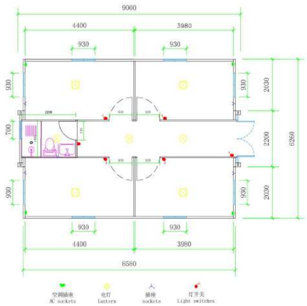
30-foot double-wing expansion room - two bedrooms, one kitchen, one bathroom B
