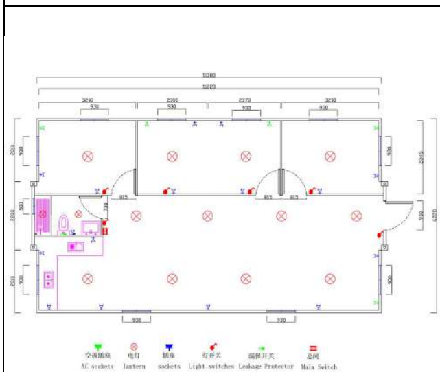
40-foot double-wing expansion room - two bedrooms, one kitchen, one bathroom, B
