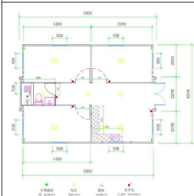
30-foot double-wing expansion room - two bedrooms, one kitchen, one bathroom A
