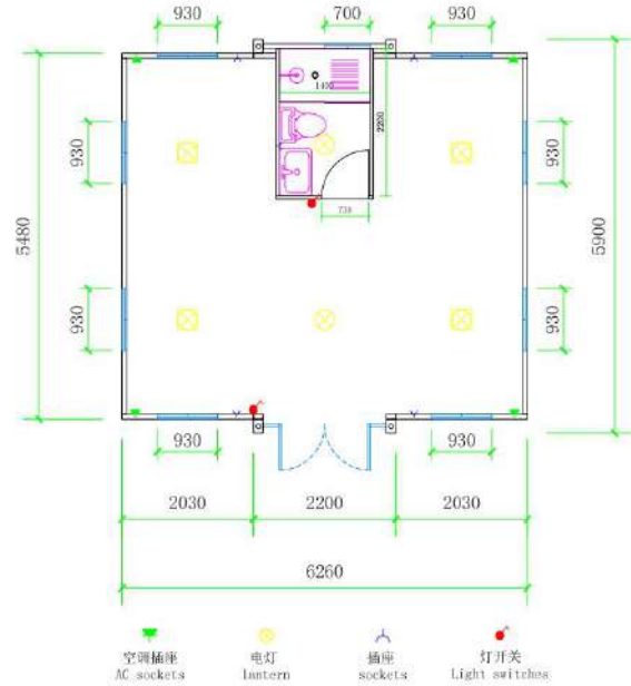
20-foot double-wing expansion home—one bathroom per room
