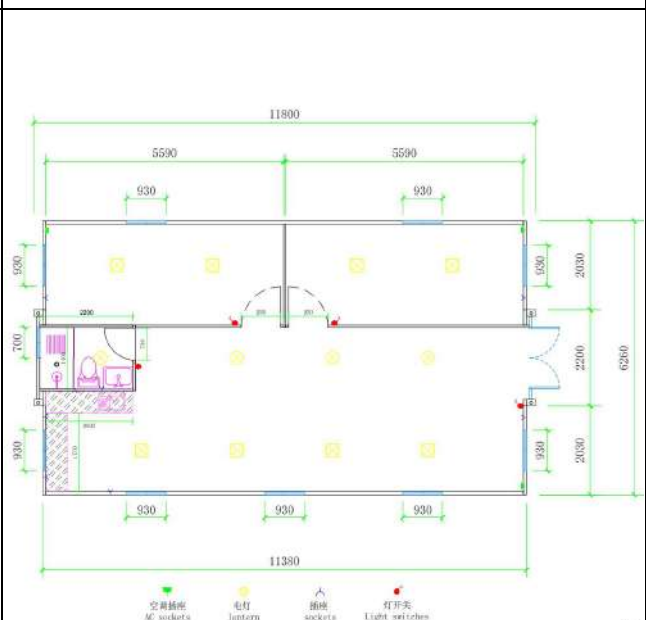
40-foot double-wing expansion home—one bathroom per unit
