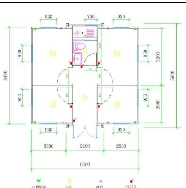
20-foot double-wing expansion room - two bedrooms, one kitchen, one bathroom B
