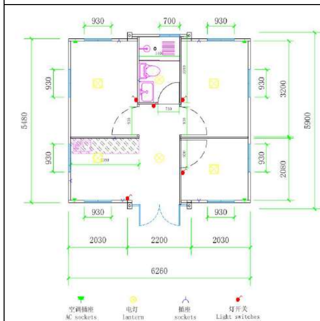
20-foot double-wing expansion room - two bedrooms, one kitchen, one bathroom A
