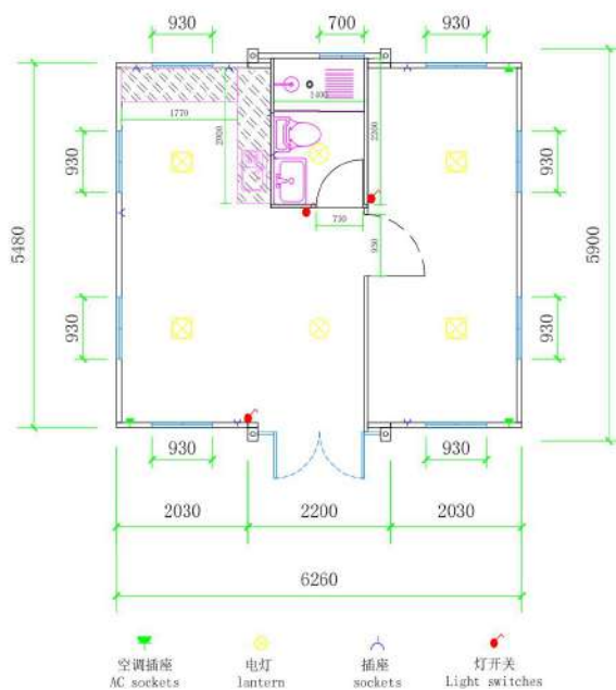
20-foot double-wing expansion room - one bedroom, one kitchen, one bathroom B
