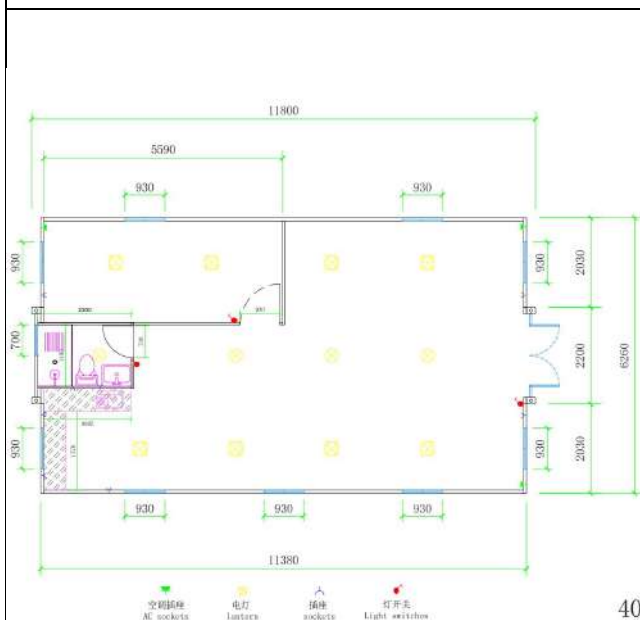
40-foot double-wing expansion room - full room
