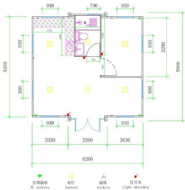
20-foot double-wing expansion room - one bedroom, one kitchen, one bathroom A
