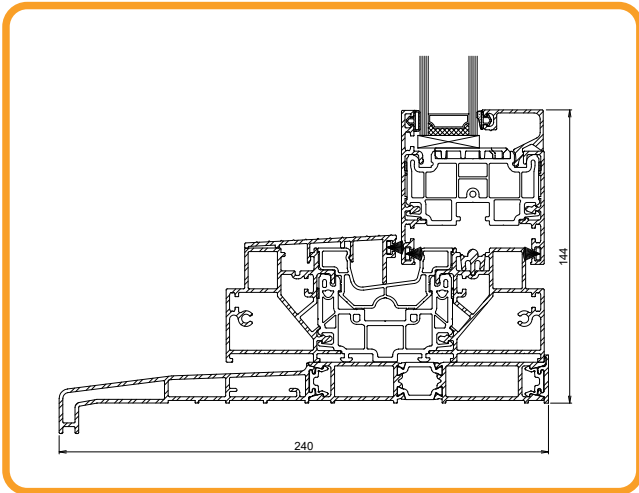
STANDARD OUTER FRAME WITH 240MM CILL
