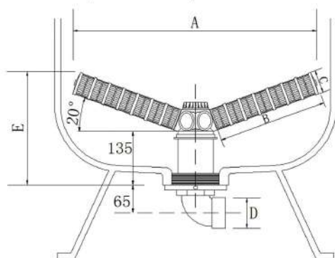
(ELBOW CONNECT)
