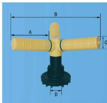
6"法兰三爪侧装上布水器 (Top mount 3 laterals diffuser 6" flange)
