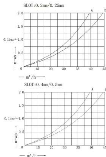
(STRAIGHT CONNECT)
