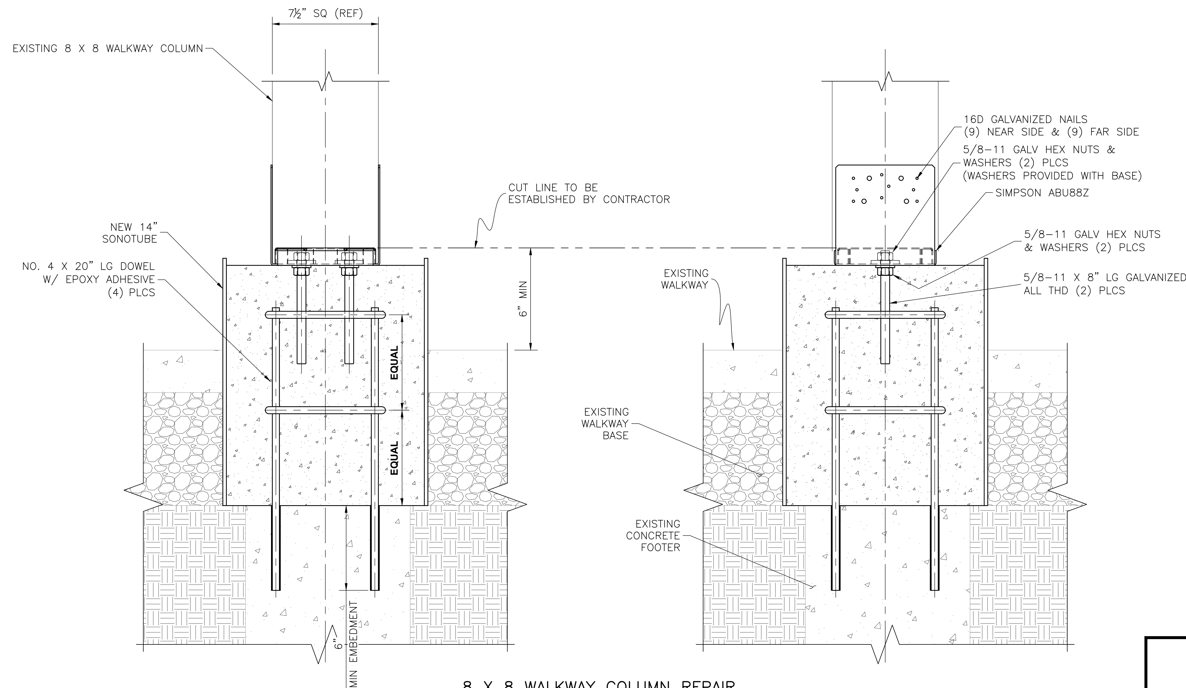
8 X 8 WALKWAY COLUMN REPAIR W/ BURIED FOOTER SCALE: 3" = 1'-0"
