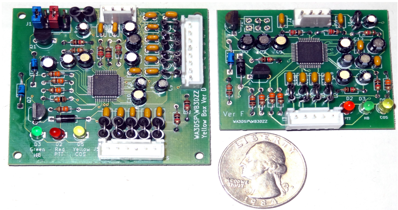
Photo of ARA-1+ FOB on the left and ARA-1 on the right. Shown in comparison to the size of a quarter.
