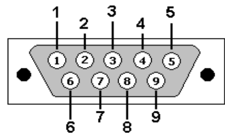
DB9 Male looking into the connector
