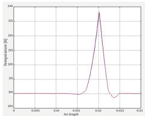
Figure 8. Temperature Rise of Fat Tissue After Radiation of 1064 nm Wavelength at the Depth of 1 cm Below the Tissue Surface
