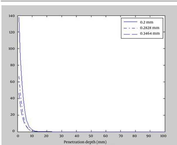
Figure 5. Absorption Versus Penetration Depth for Various Beam Radiuses of 980 nm at Fixed Power of 10 Watt
