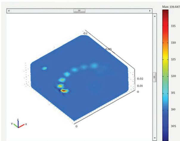
Figure 6. Temperature Rise Following the Irradiation of 1064 nm Wavelength at Power of 15 Watt
