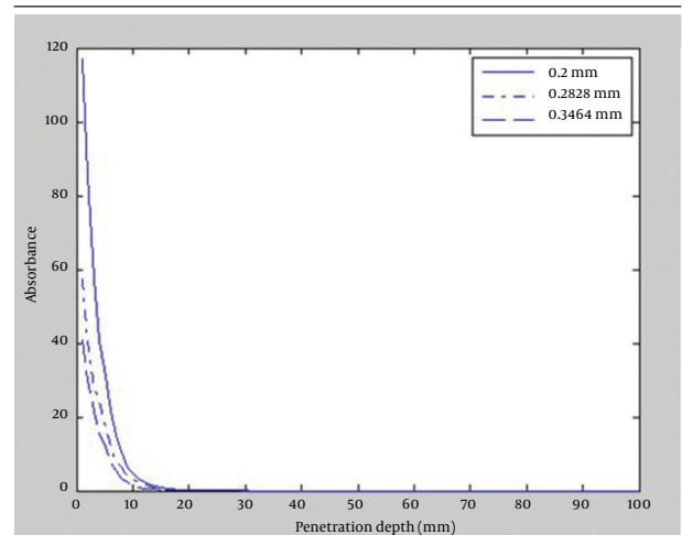
Figure 4. Absorption Versus Penetration Depth for Various Radiuses of 1064 nm at Fixd Power of 10 Watt
