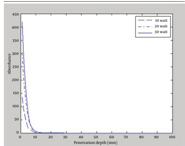
Figure 3. Absorption Versus Penetration Depth for Various Powers of 980 nm Wavelength and Fixed Beam Radius of 200 μm
