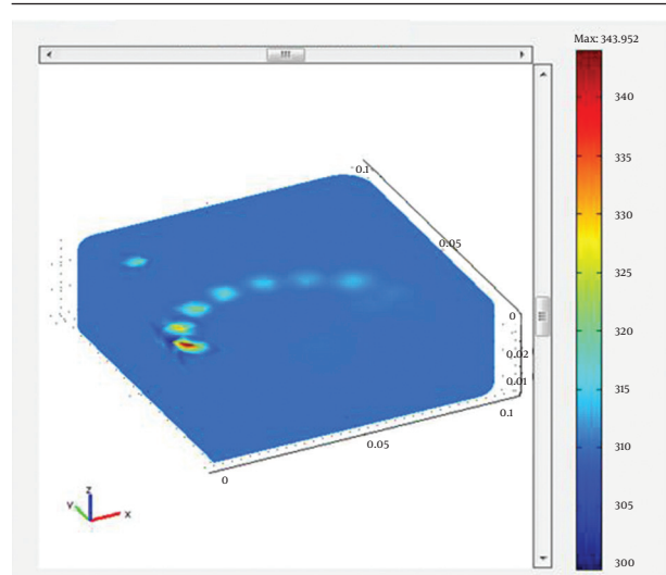
Figure 7. Temperature Rise Following the Irradiation of 980 nm Wavelength at Power of 15 Watt
