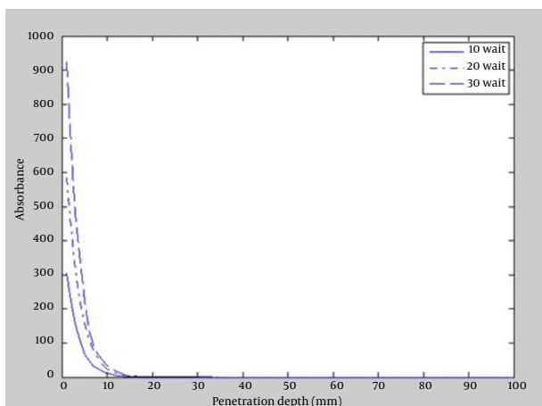
Figure 2. Absorption Versus Penetration Depth for Various Powers of 1064 nm Wavelength and Fixed Beam Radius of 200 μm
