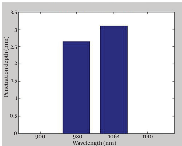
Figure 1. Penetration Depth for Wavelengths Under Study
