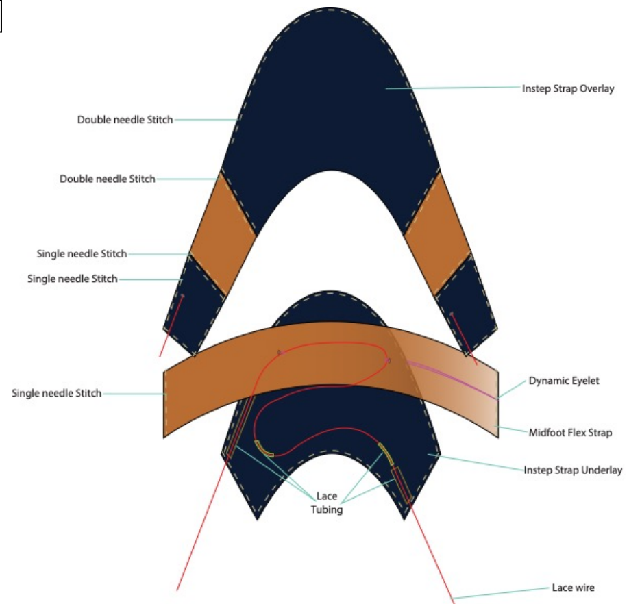
TOP VIEW OF INSTEP STRAP
