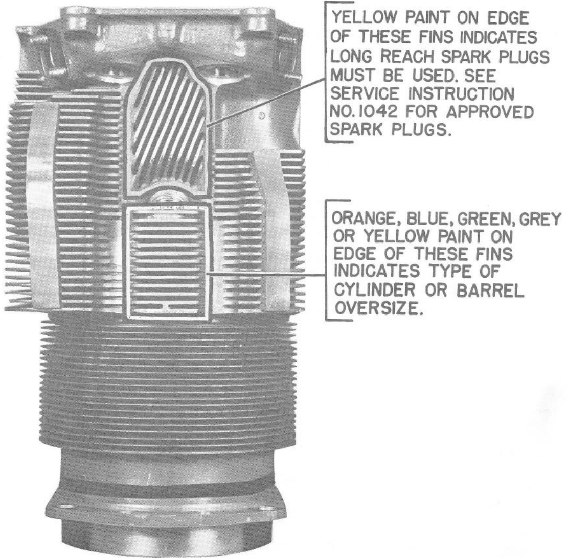
Cylinder Assembly Showing Color Coded Areas
