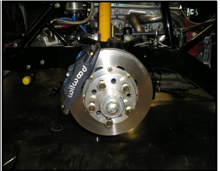
WILWOOD 4 PISTON CALIPER, TUBULAR SPINDLE BILLET STEEL OR ALUMINUM HUBS
