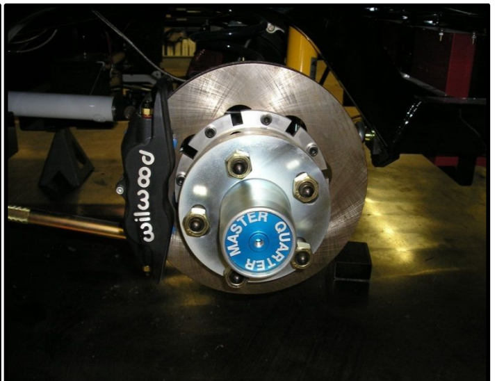
9 inch FLOATER REAREND WITH BILLET ALUM HUBS
