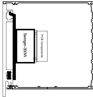
HORTON FULL ACCESS HEADER MOUNTING OPTION Part # Horton Mount
