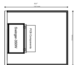
LOW PROFILE HEADER MOUNTING OPTION Part # Low Profile Mount
