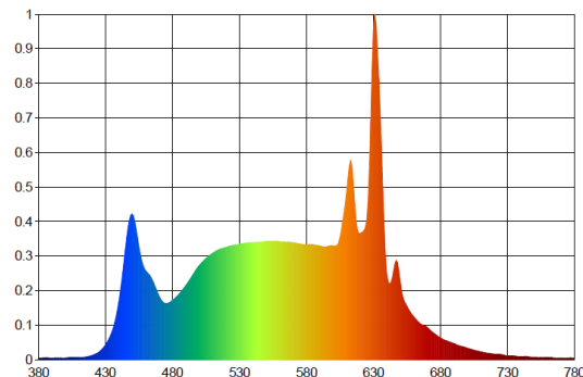
COLOUR DISTRIBUTION Nm for 4000K
