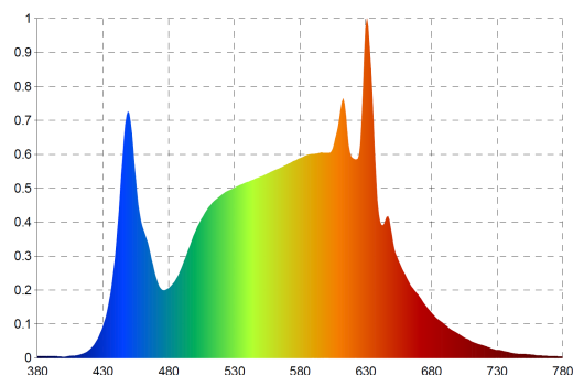
COLOUR DISTRIBUTION Nm for 4000K
