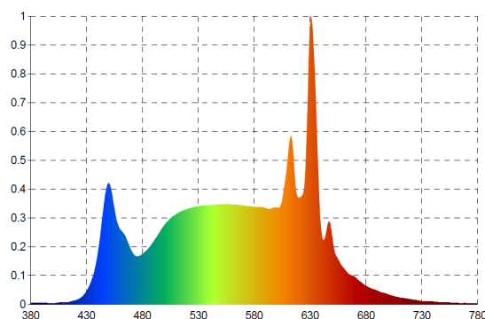
COLOUR DISTRIBUTION Nm for 4000K
