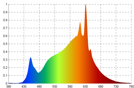
COLOUR DISTRIBUTION Nm for 3000K
