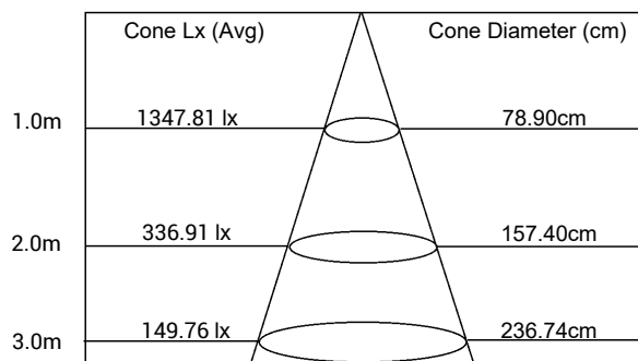
LIGHT DISTRIBUTION for Medium 36°
