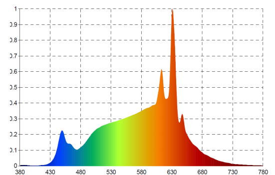
COLOUR DISTRIBUTION Nm for 3000K
