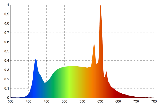
COLOUR DISTRIBUTION Nm for 3000K
