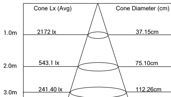
LIGHT DISTRIBUTION for Spot 20°
