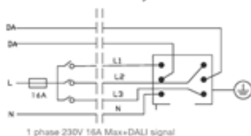
3 circuit DALI track system
