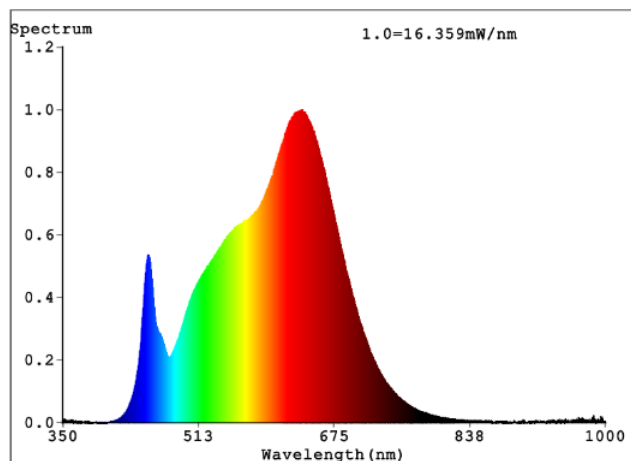
COLOUR DISTRIBUTION Nm for 3000K
