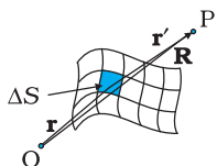
Surface charge \Delta Q = \sigma \Delta S
