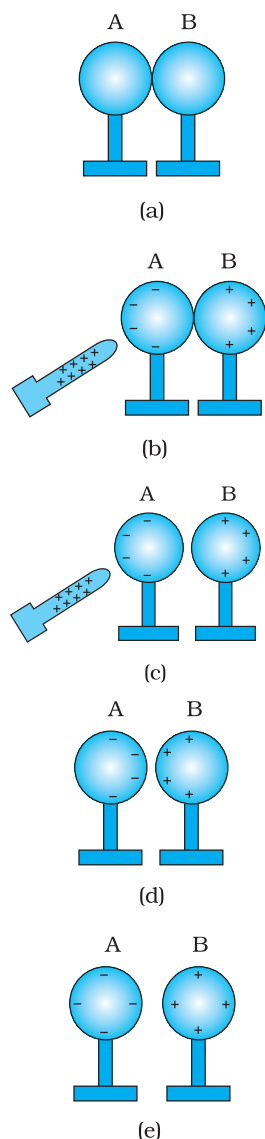
FIGURE 1.4 Charging by induction.
