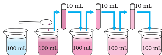
Fig. 1.2: Estimating how small are the particles of matter. With every dilution, though the colour becomes lighter, it is still visible.
