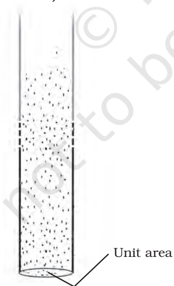
Fig. 11.17 : Atmospheric pressure is the force of gravity on air in a column of unit area
