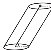
Fig 11.27 (This is not a right circular cylinder)
