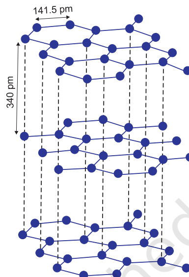
Fig 11.4 The structure of graphite
