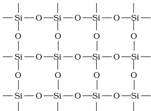
Fig. 11.6 Three dimensional structure of \text{SiO}_2
