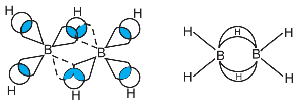
Fig.11.2(b) Bonding in diborane. Each B atom uses sp^3 hybrids for bonding. Out of the four sp^3 hybrids on each B atom, one is without an electron shown in broken lines. The terminal B-H bonds are normal 2-centre-2-electron bonds but the two bridge bonds are 3-centre-2-electron bonds. The 3-centre-2-electron bridge bonds are also referred to as banana bonds.
