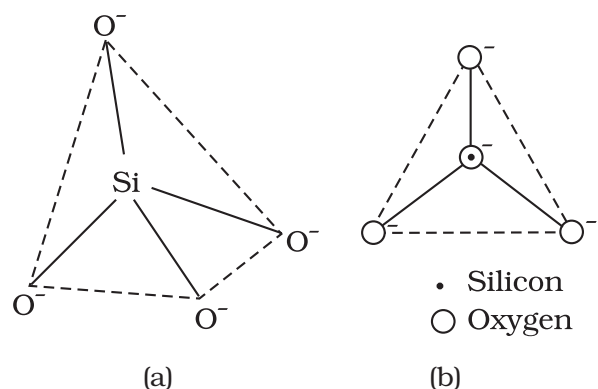
Fig. 11.7 (a) Tetrahedral structure of \text{SiO}_4^{4-} anion; (b) Representation of \text{SiO}_4^{4-} unit
