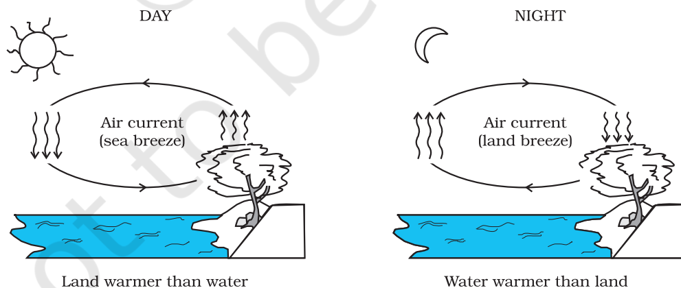
Fig. 11.17 Convection cycles.
