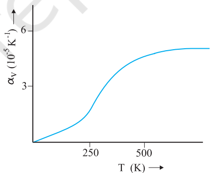
Fig. 11.6 Coefficient of volume expansion of copper as a function of temperature.
